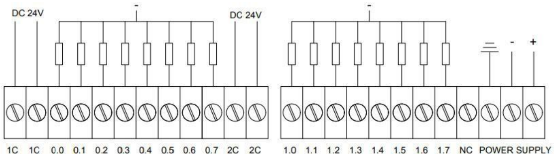
Figure 2.6 DO wiring diagram of GCAN-PLC-326E/R series
