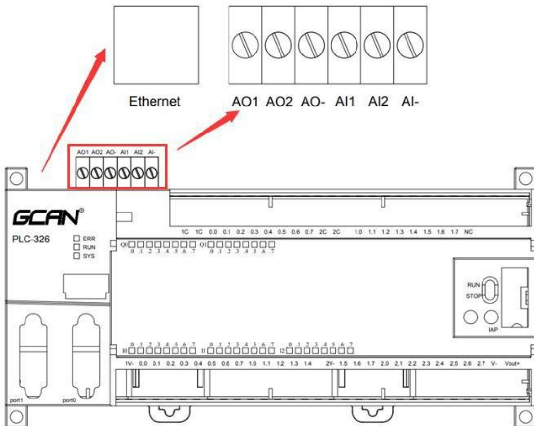
Figure 2.7 AI/AO terminal diagram of GCAN-PLC-326E/R series
