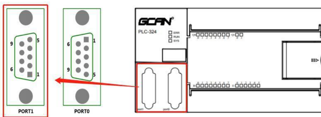
Figure 2.3 PORT0, PORT1 interface of GCAN-PLC-326E/R series
