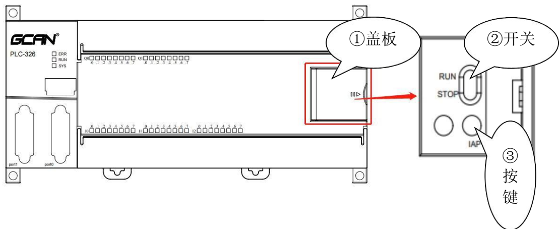
4.1 Physical picture of running switch and reset button
