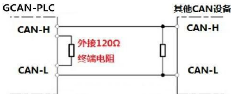
Figure 3.2 Connection between GCAN-PLC-326E/R series modules and other CAN node devices
