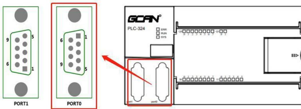
Figure 2.2 PORT0, PORT1 interface of GCAN-PLC-326E/R series
